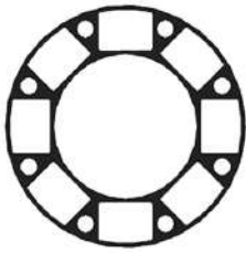
SC-11 DISCO SEPARADOR VOLVO EDC BI-DISCO 2MM
